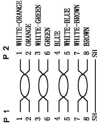
WIRING DIAGRAM
